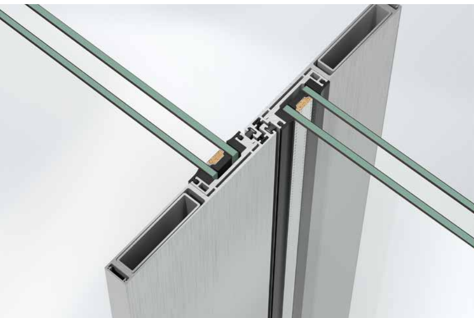
(Double-track sliding door (Interlock section))
